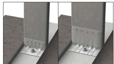
Figure C Kwik-Bolts
